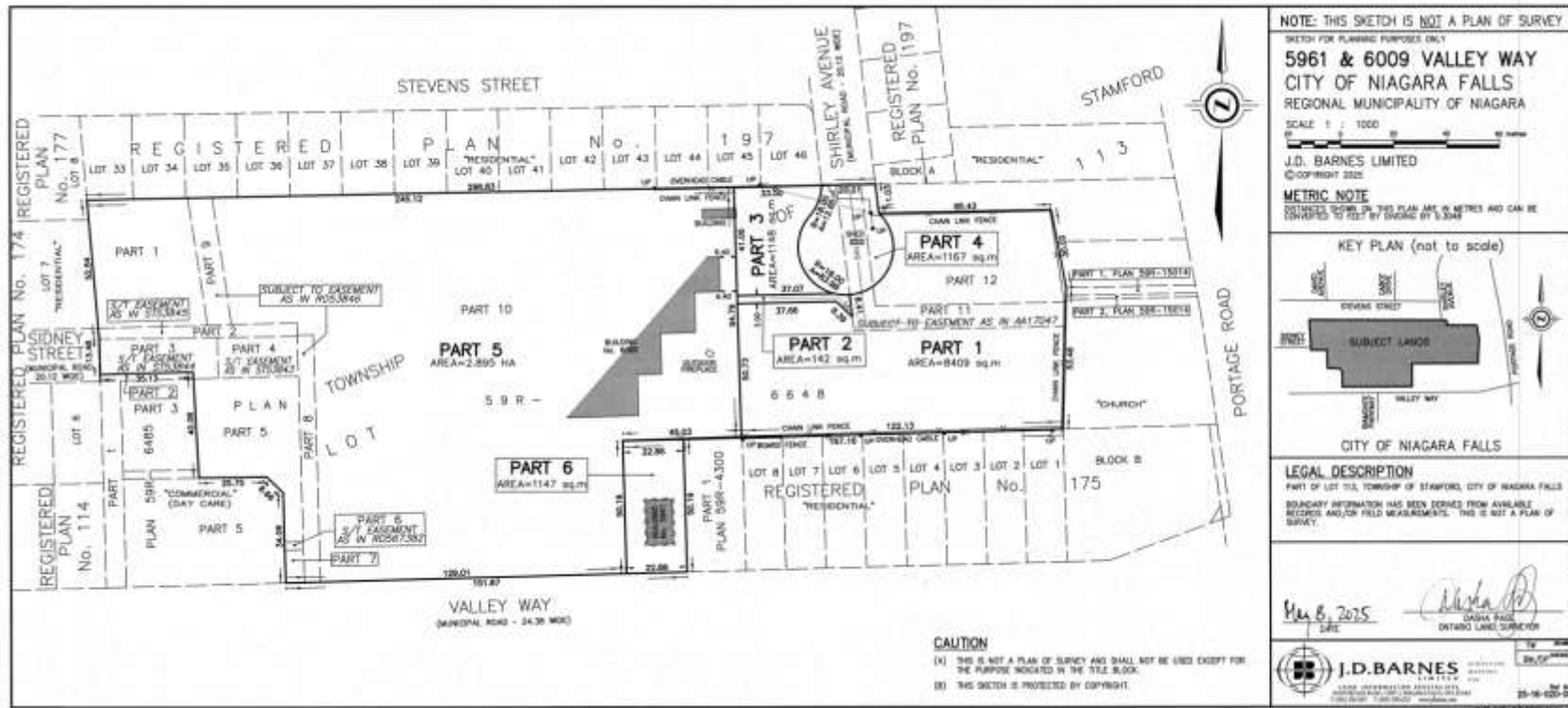
Figure 6: Survey Sketch
